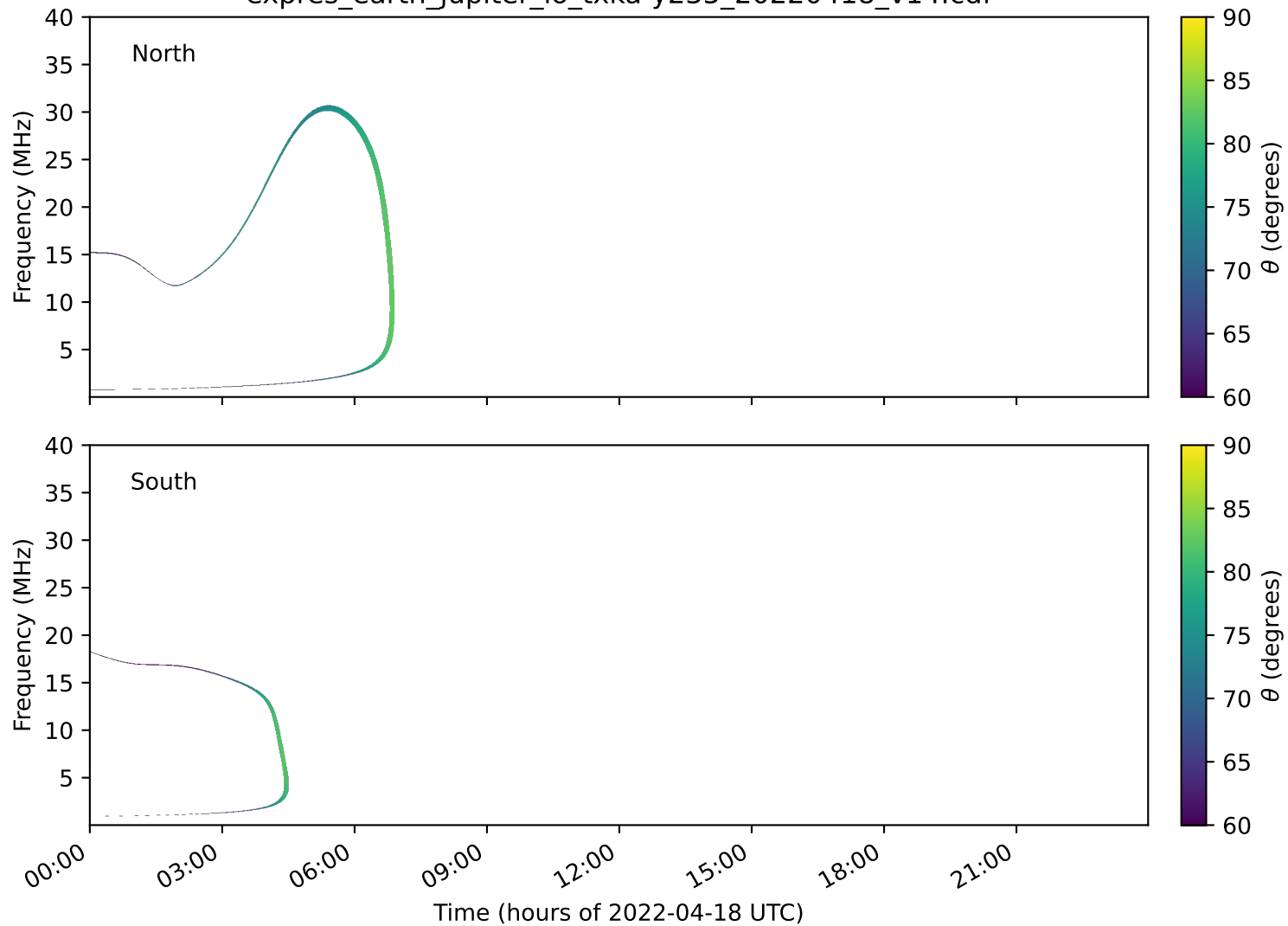
expres_earth_jupiter_io_txka-y235_20220418_v14.cdf
