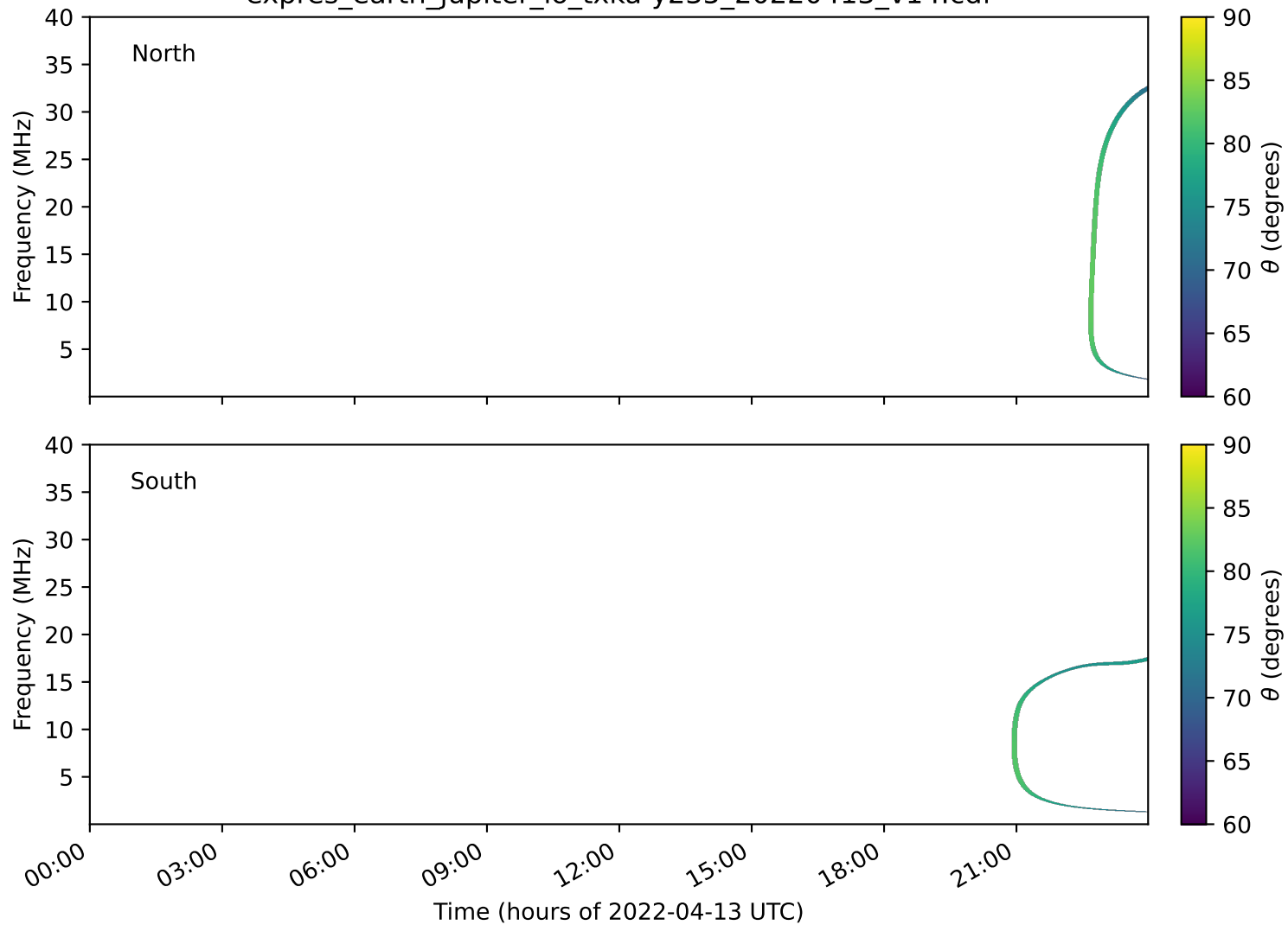
expres_earth_jupiter_io_txka-y235_20220413_v14.cdf
