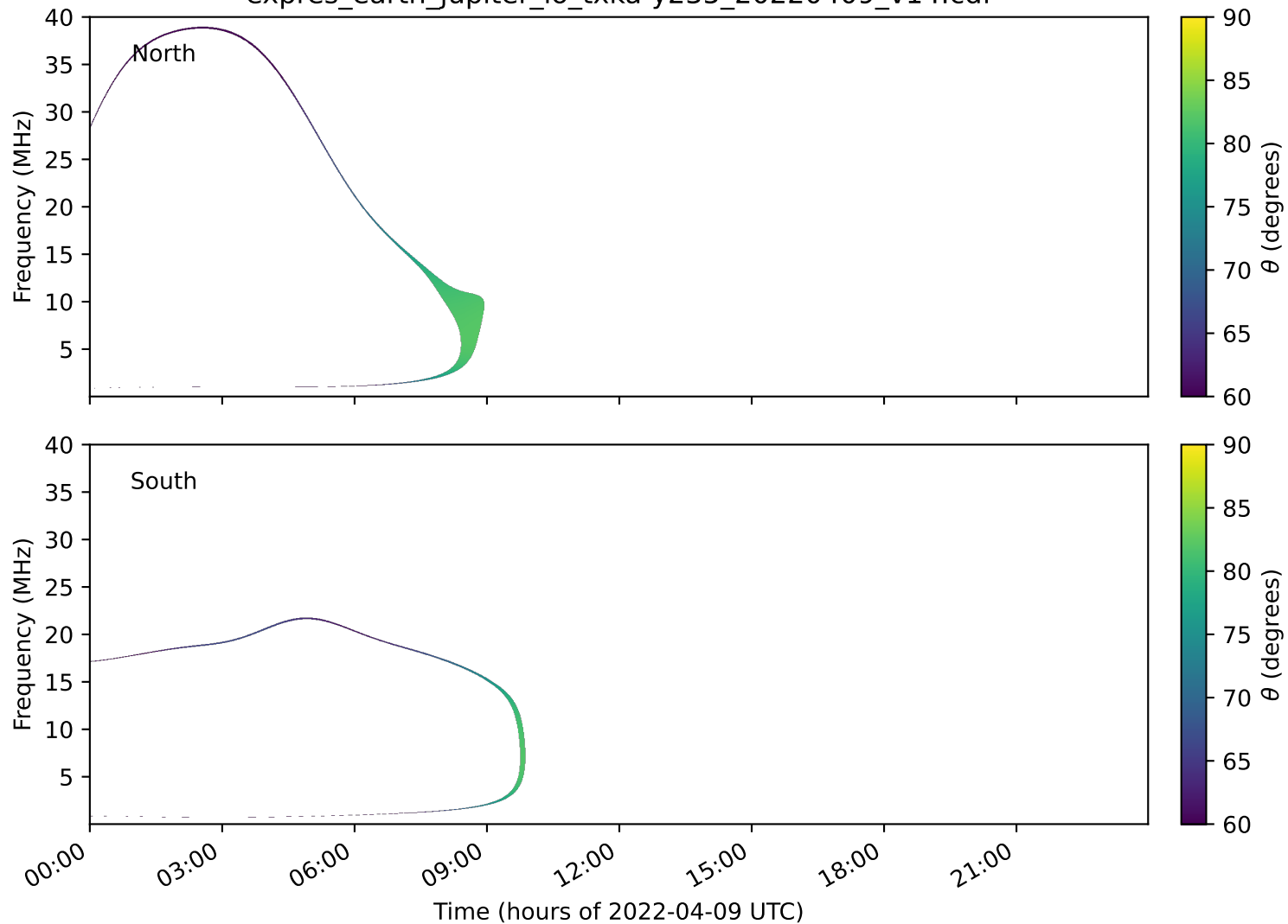
expres_earth_jupiter_io_txka-y235_20220409_v14.cdf
