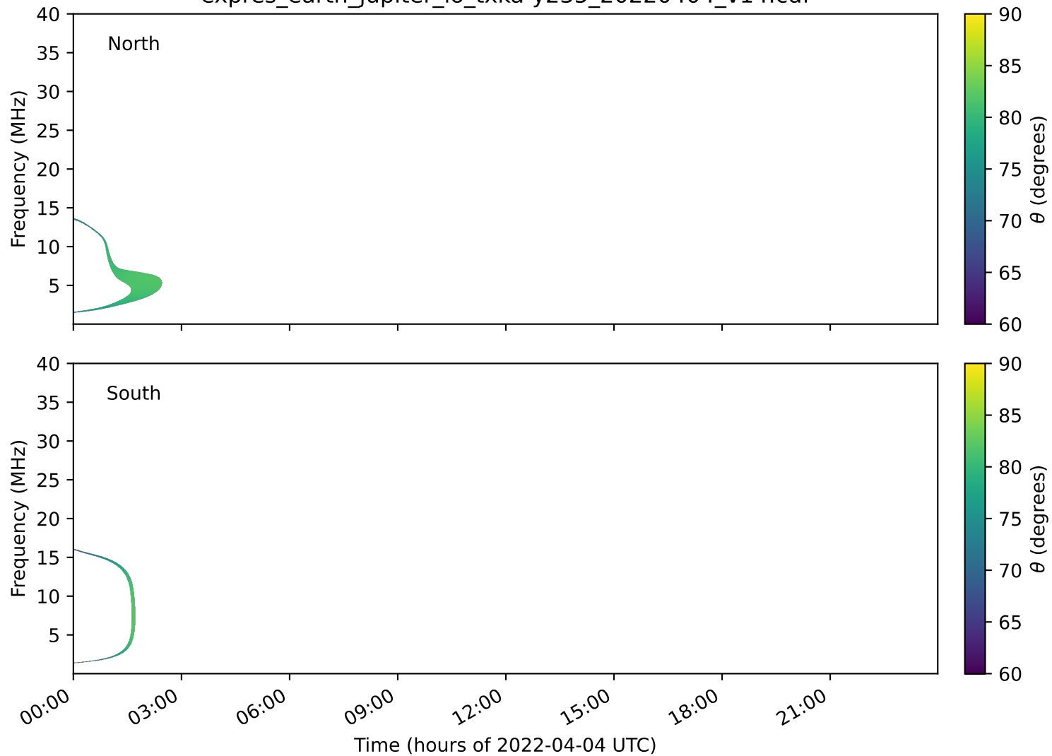
expres_earth_jupiter_io_txka-y235_20220404_v14.cdf
