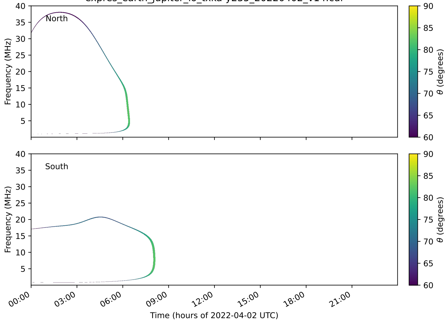
expres_earth_jupiter_io_txka-y235_20220402_v14.cdf
