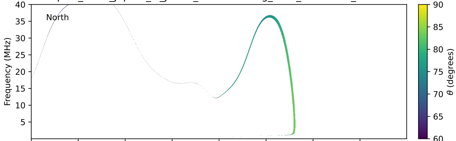
expres_earth_jupiter_io_jrm33_lossc-wid1deg_3kev_20220430_v11.cdf
