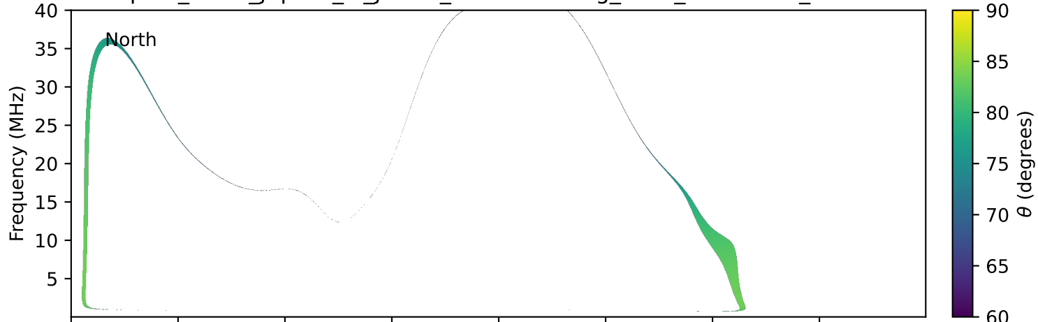
expres_earth_jupiter_io_jrm33_lossc-wid1deg_3kev_20220421_v11.cdf
