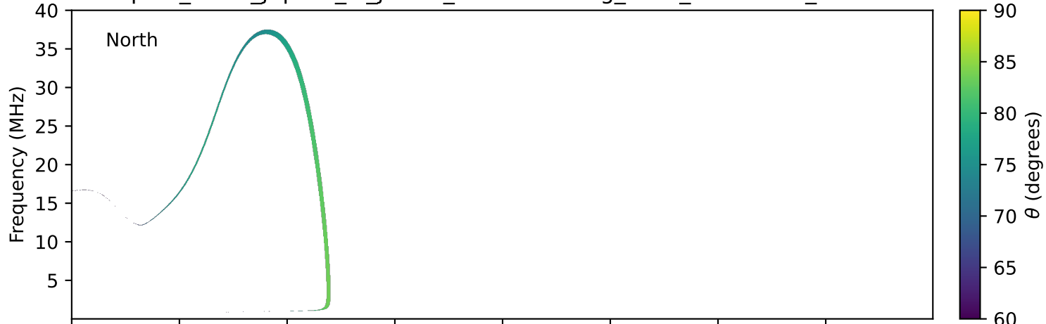
expres_earth_jupiter_io_jrm33_lossc-wid1deg_3kev_20220418_v11.cdf
