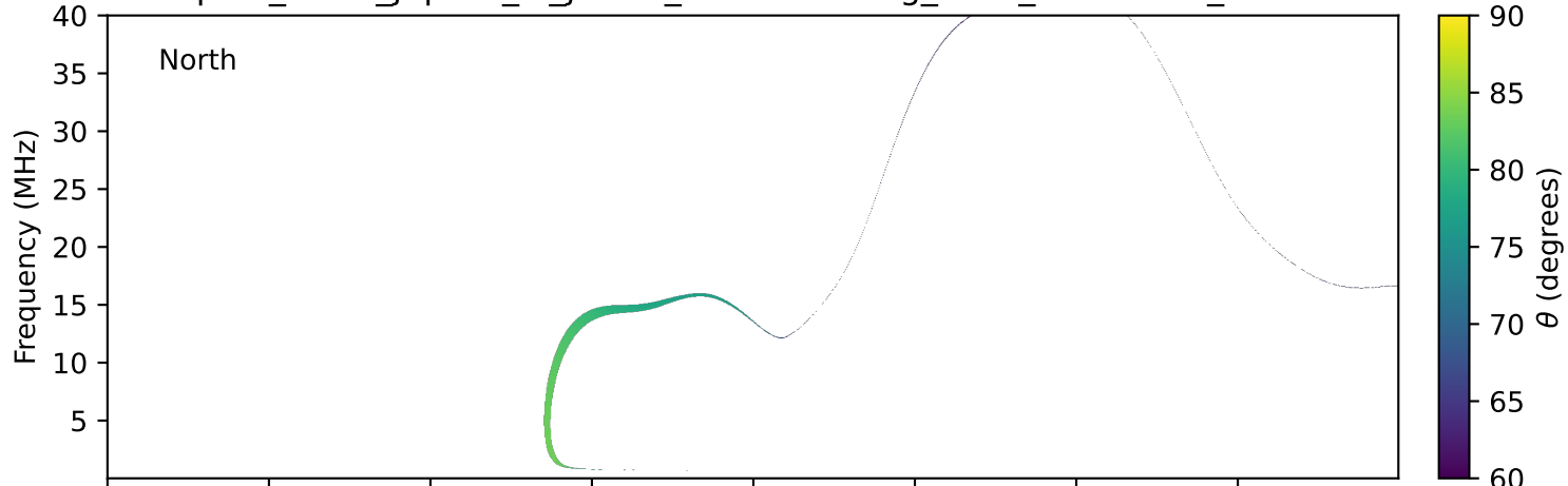
expres_earth_jupiter_io_jrm33_lossc-wid1deg_3kev_20220410_v11.cdf
