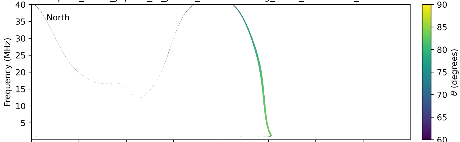
expres_earth_jupiter_io_jrm33_lossc-wid1deg_3kev_20220407_v11.cdf
