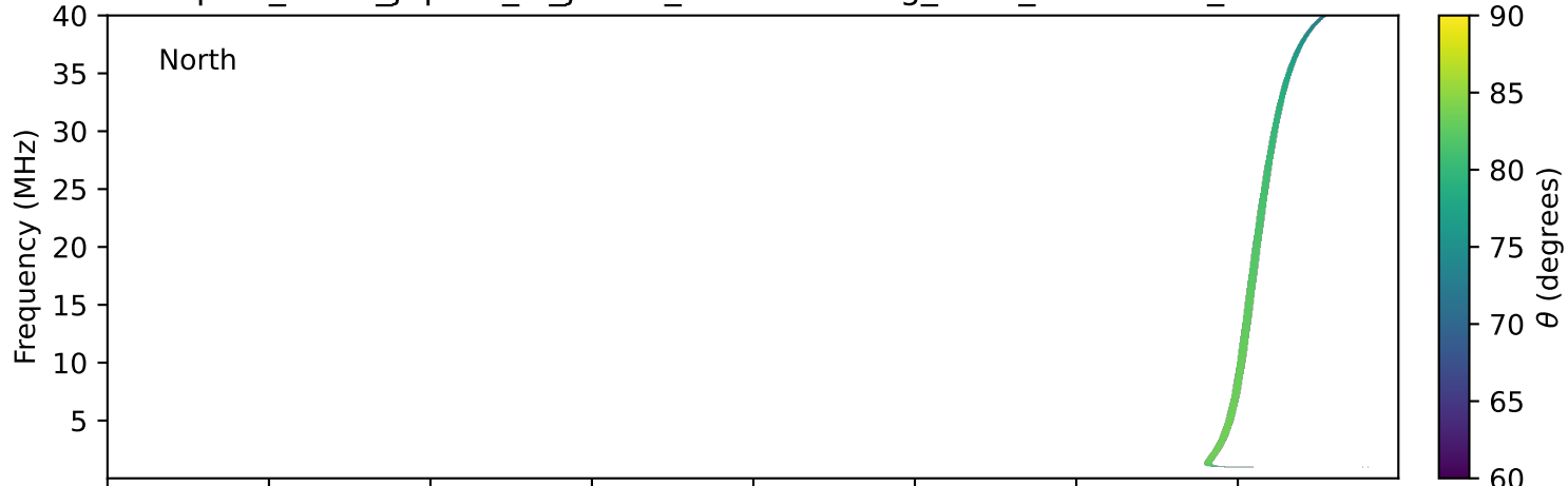
expres_earth_jupiter_io_jrm33_lossc-wid1deg_3kev_20220406_v11.cdf
