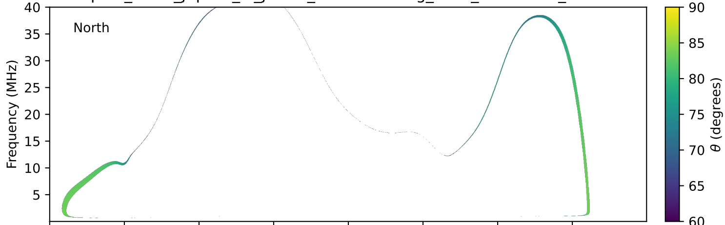
expres_earth_jupiter_io_jrm33_lossc-wid1deg_3kev_20220405_v11.cdf
