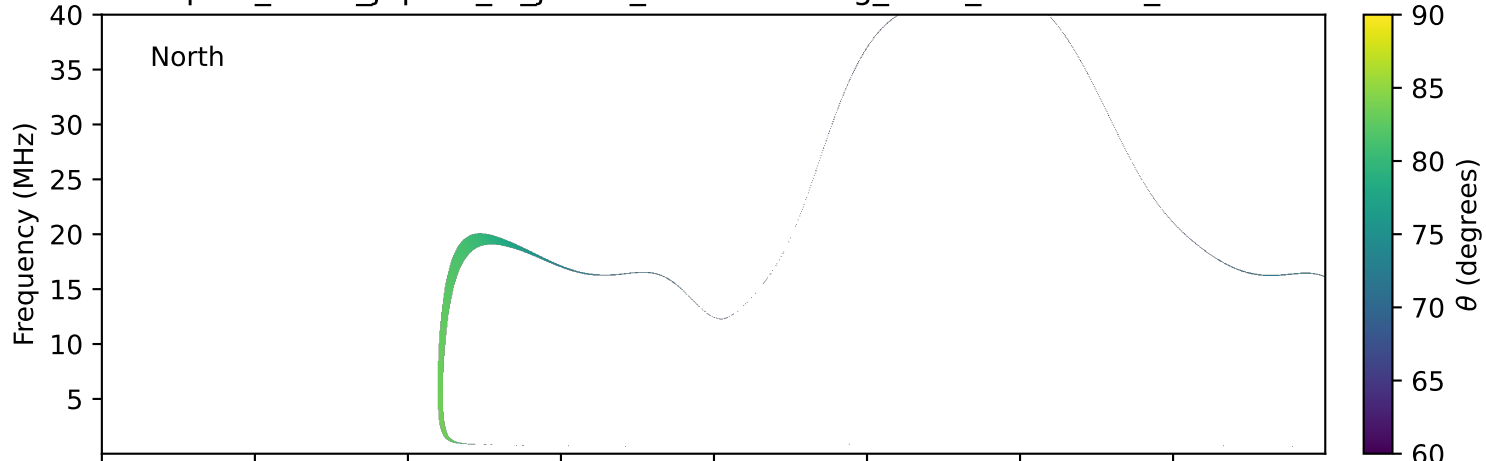
expres_earth_jupiter_io_jrm33_lossc-wid1deg_3kev_20220403_v11.cdf
