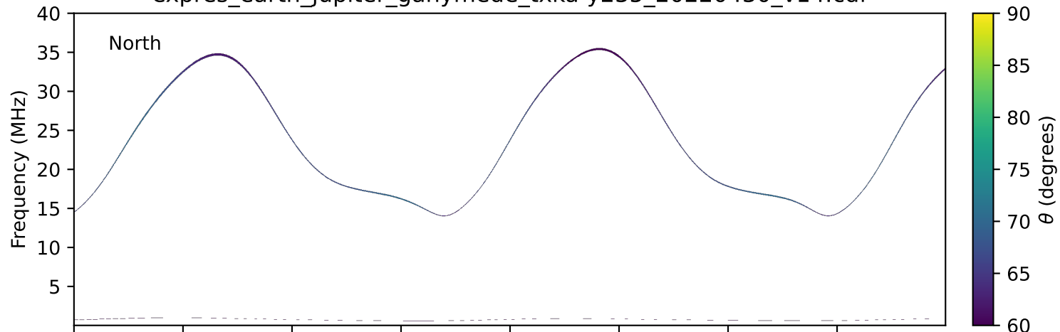
expres_earth_jupiter_ganymede_txka-y235_20220430_v14.cdf
