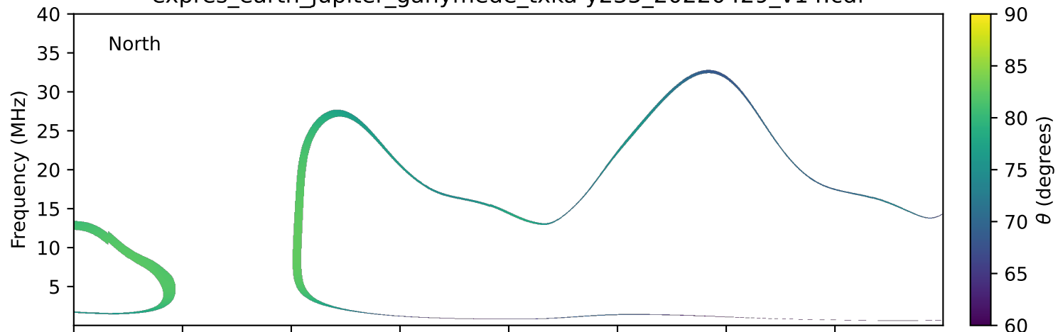
expres_earth_jupiter_ganymede_txka-y235_20220429_v14.cdf
