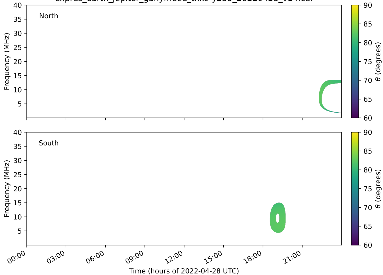
expres_earth_jupiter_ganymede_txka-y235_20220428_v14.cdf
