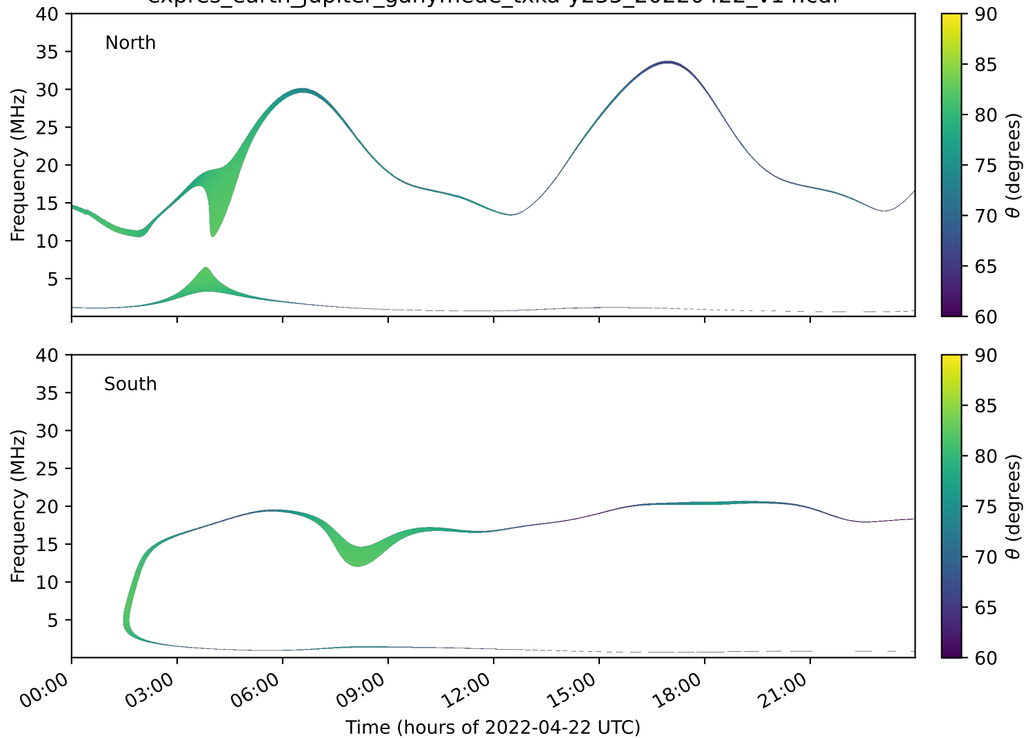
expres_earth_jupiter_ganymede_txka-y235_20220422_v14.cdf
