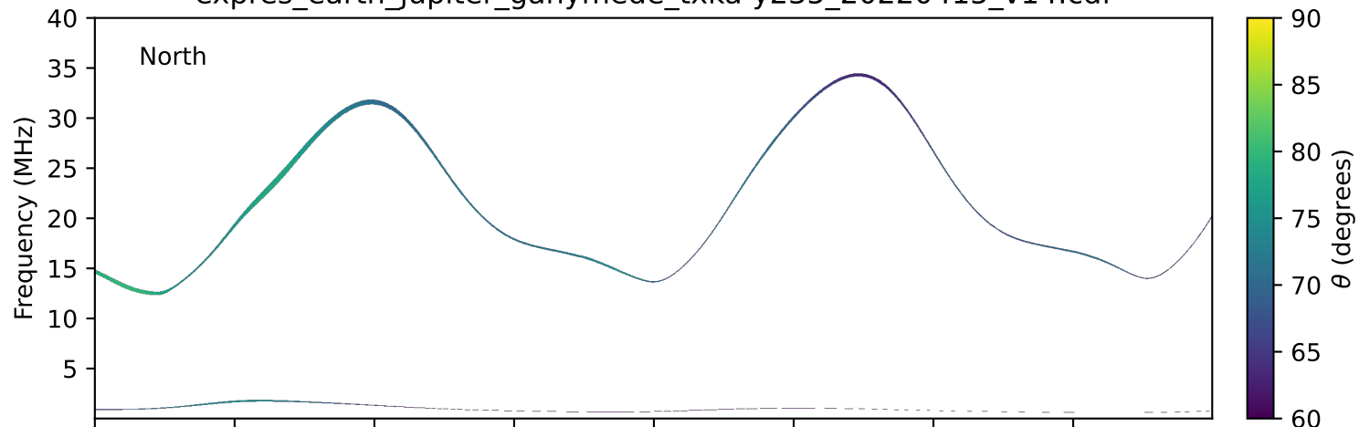
expres_earth_jupiter_ganymede_txka-y235_20220415_v14.cdf
