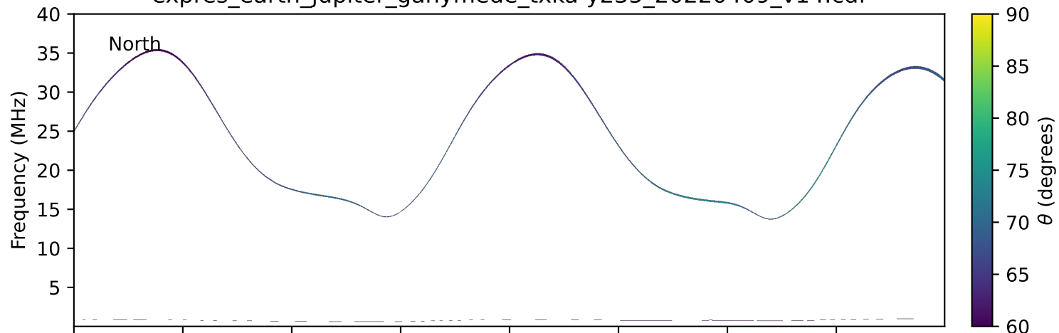
expres_earth_jupiter_ganymede_txka-y235_20220409_v14.cdf
