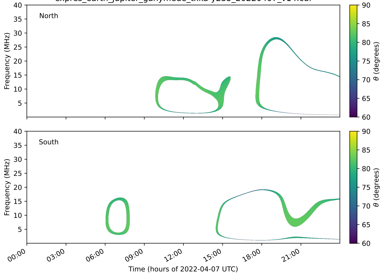
expres_earth_jupiter_ganymede_txka-y235_20220407_v14.cdf
