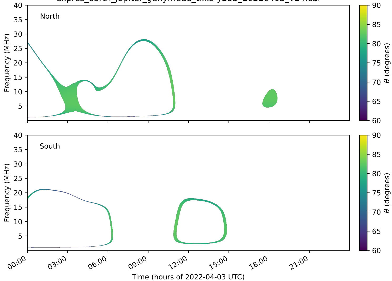
expres_earth_jupiter_ganymede_txka-y235_20220403_v14.cdf
