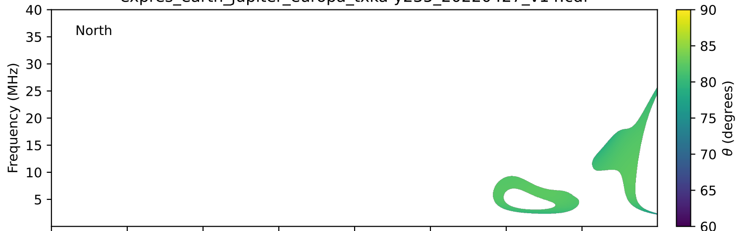
expres_earth_jupiter_europa_txka-y235_20220427_v14.cdf
