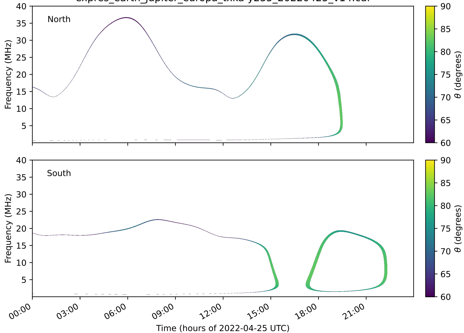
expres_earth_jupiter_europa_txka-y235_20220425_v14.cdf
