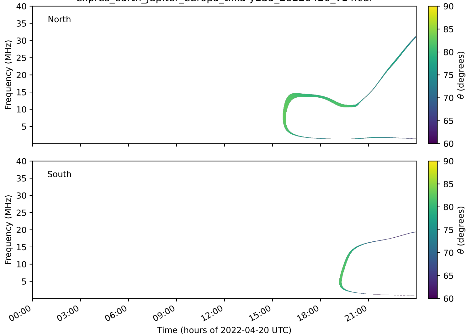
expres_earth_jupiter_europa_txka-y235_20220420_v14.cdf
