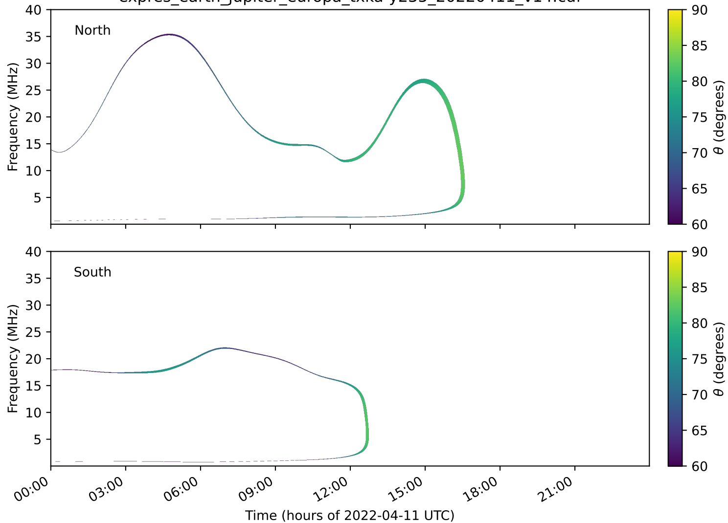
expres_earth_jupiter_europa_txka-y235_20220411_v14.cdf
