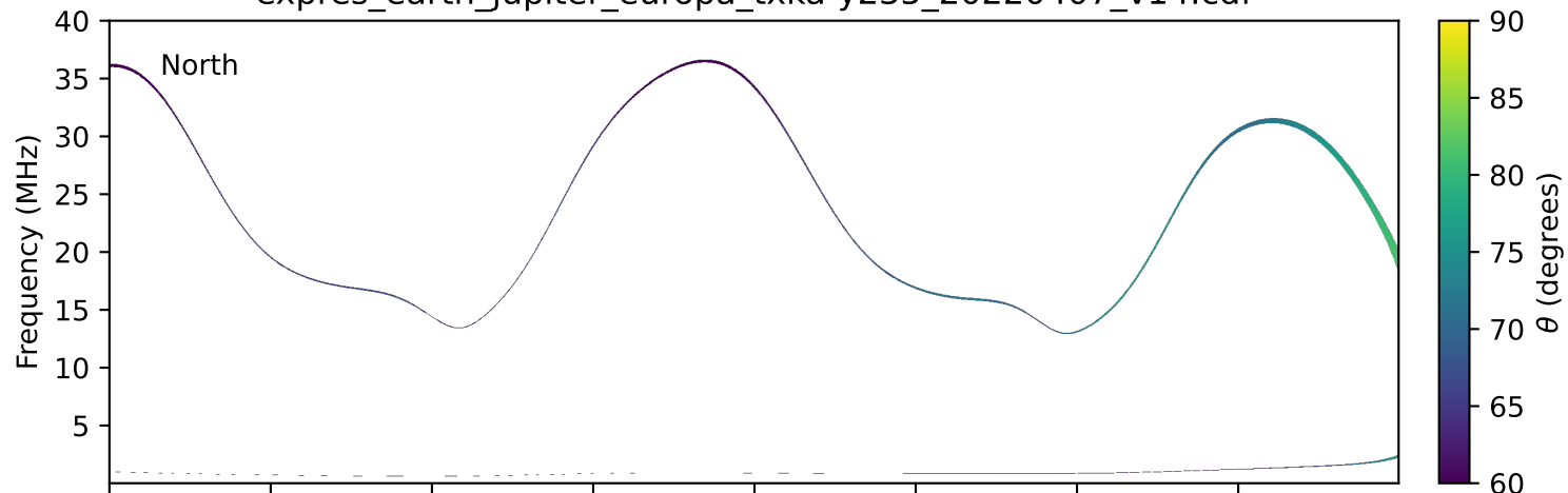
expres_earth_jupiter_europa_txka-y235_20220407_v14.cdf
