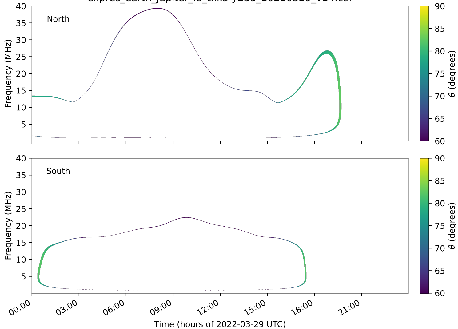
expres_earth_jupiter_io_txka-y235_20220329_v14.cdf
