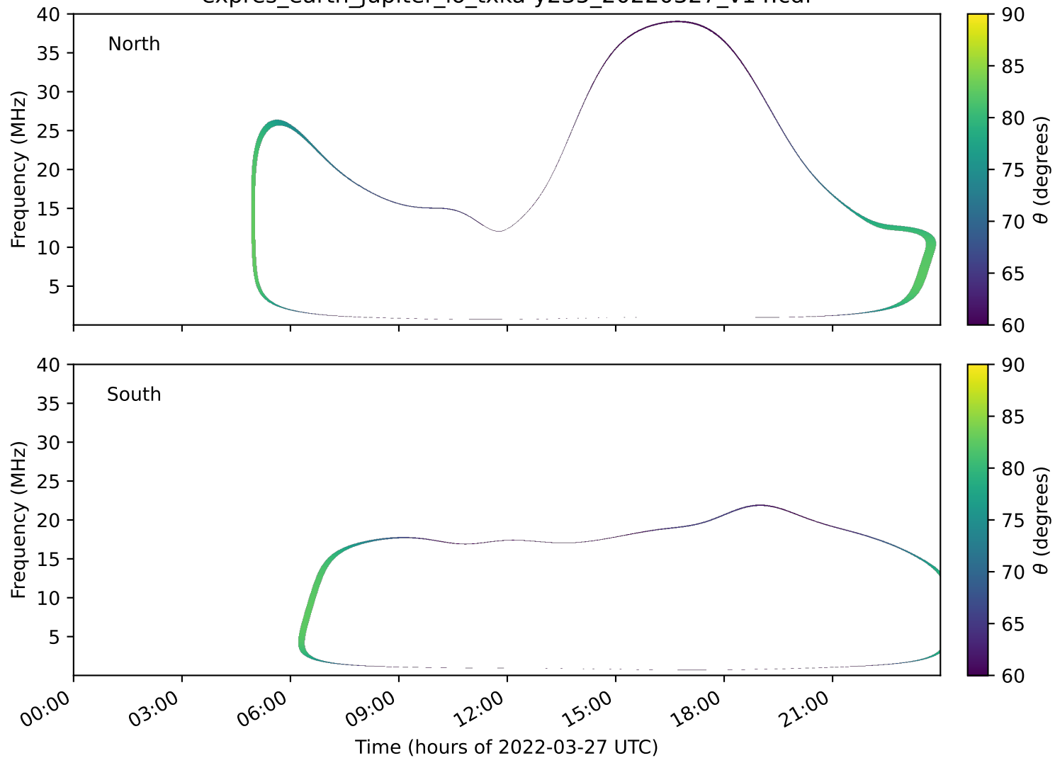
expres_earth_jupiter_io_txka-y235_20220327_v14.cdf
