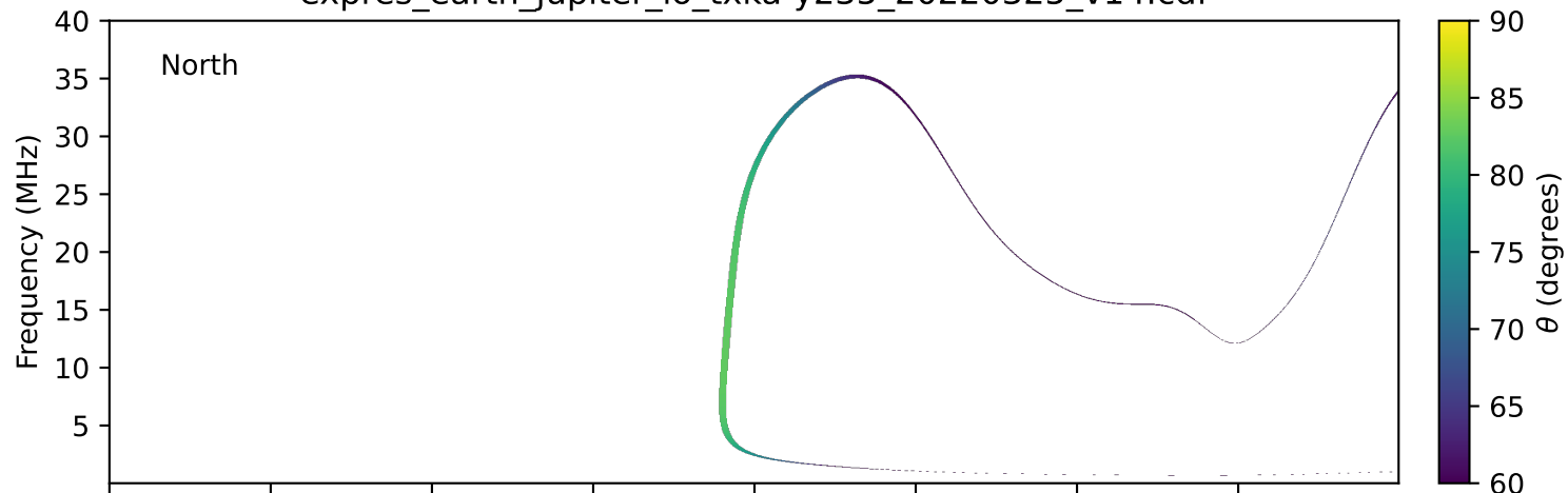
expres_earth_jupiter_io_txka-y235_20220325_v14.cdf
