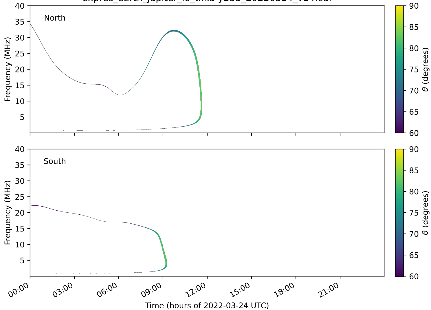
expres_earth_jupiter_io_txka-y235_20220324_v14.cdf
