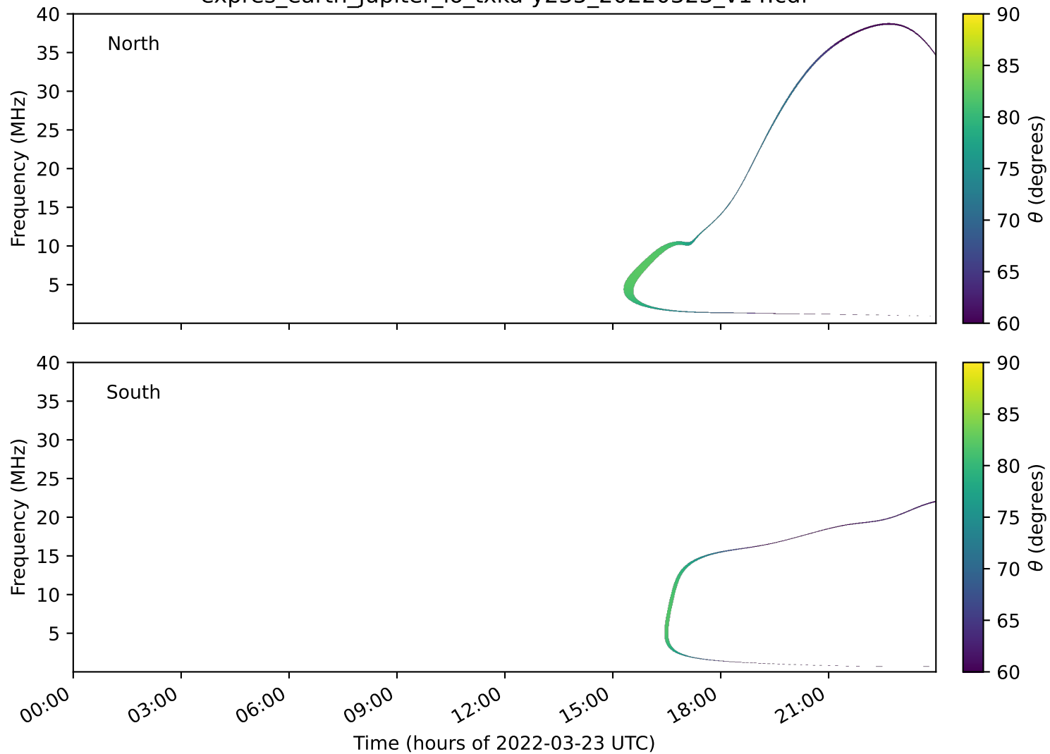
expres_earth_jupiter_io_txka-y235_20220323_v14.cdf
