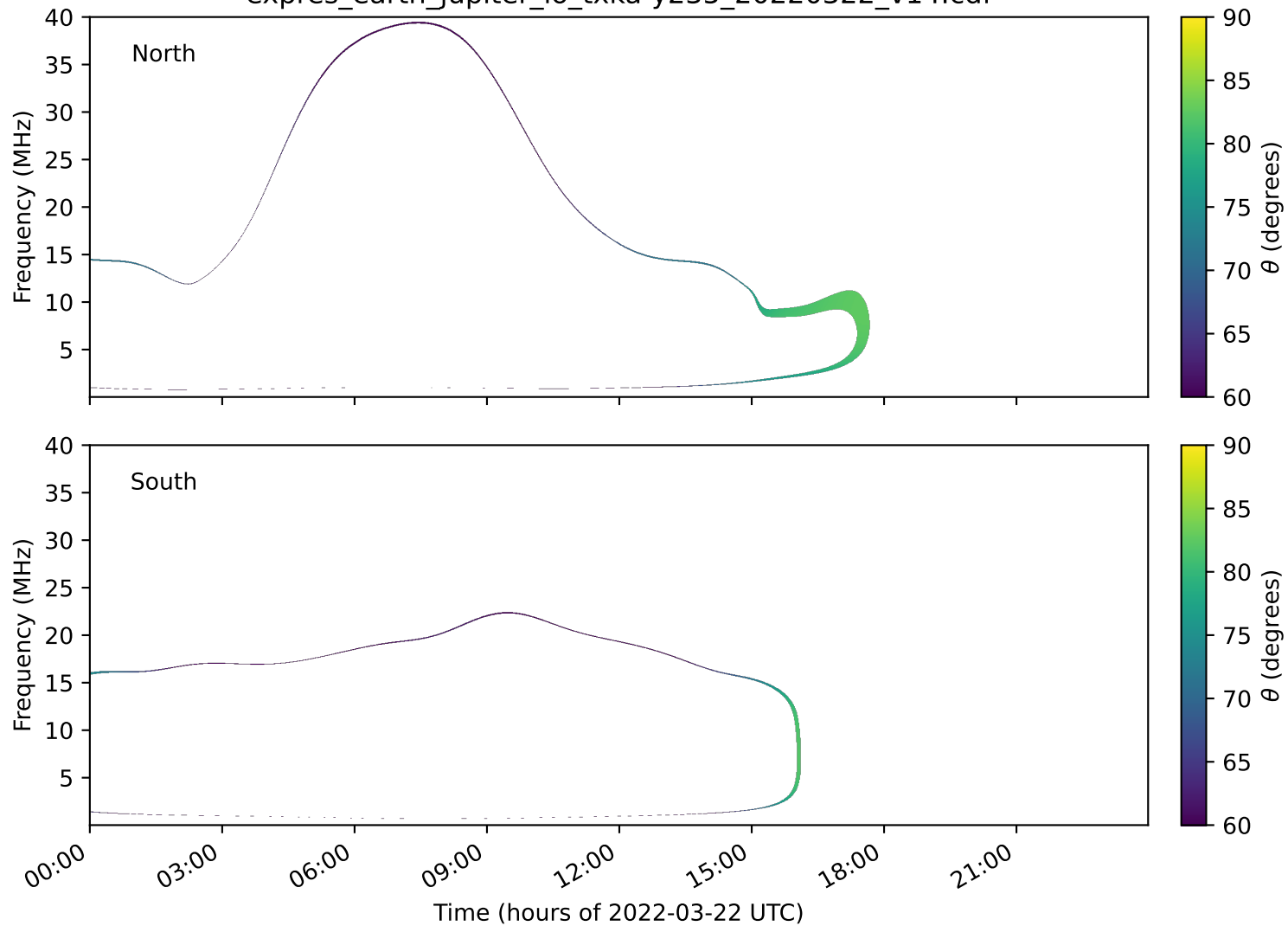
expres_earth_jupiter_io_txka-y235_20220322_v14.cdf
