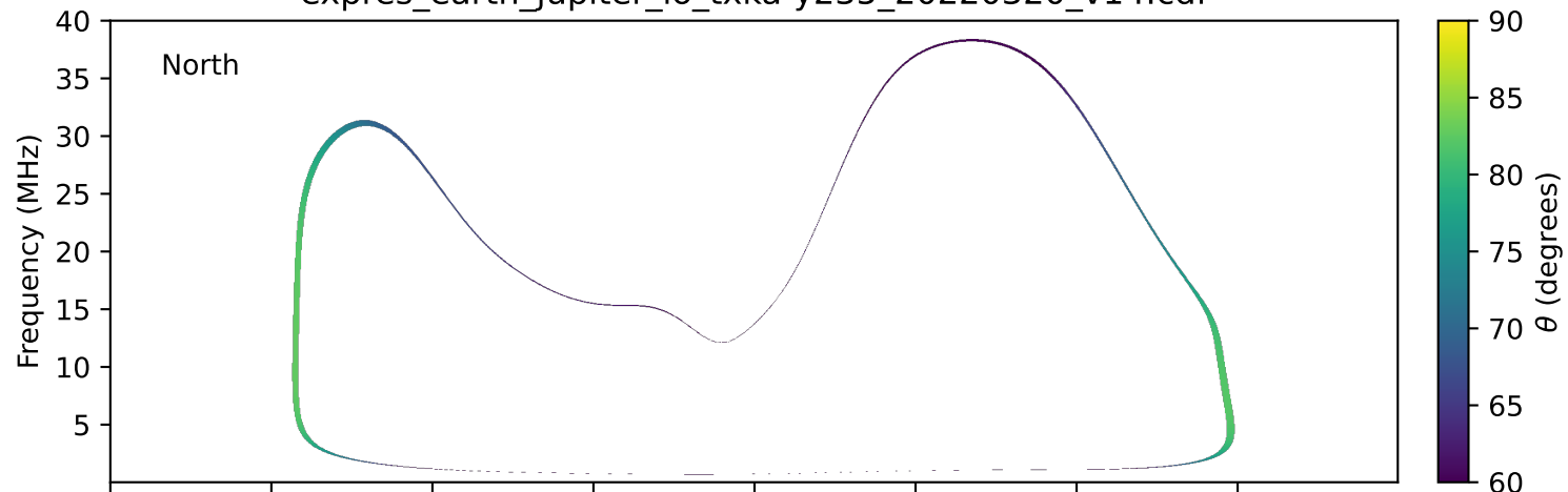
expres_earth_jupiter_io_txka-y235_20220320_v14.cdf
