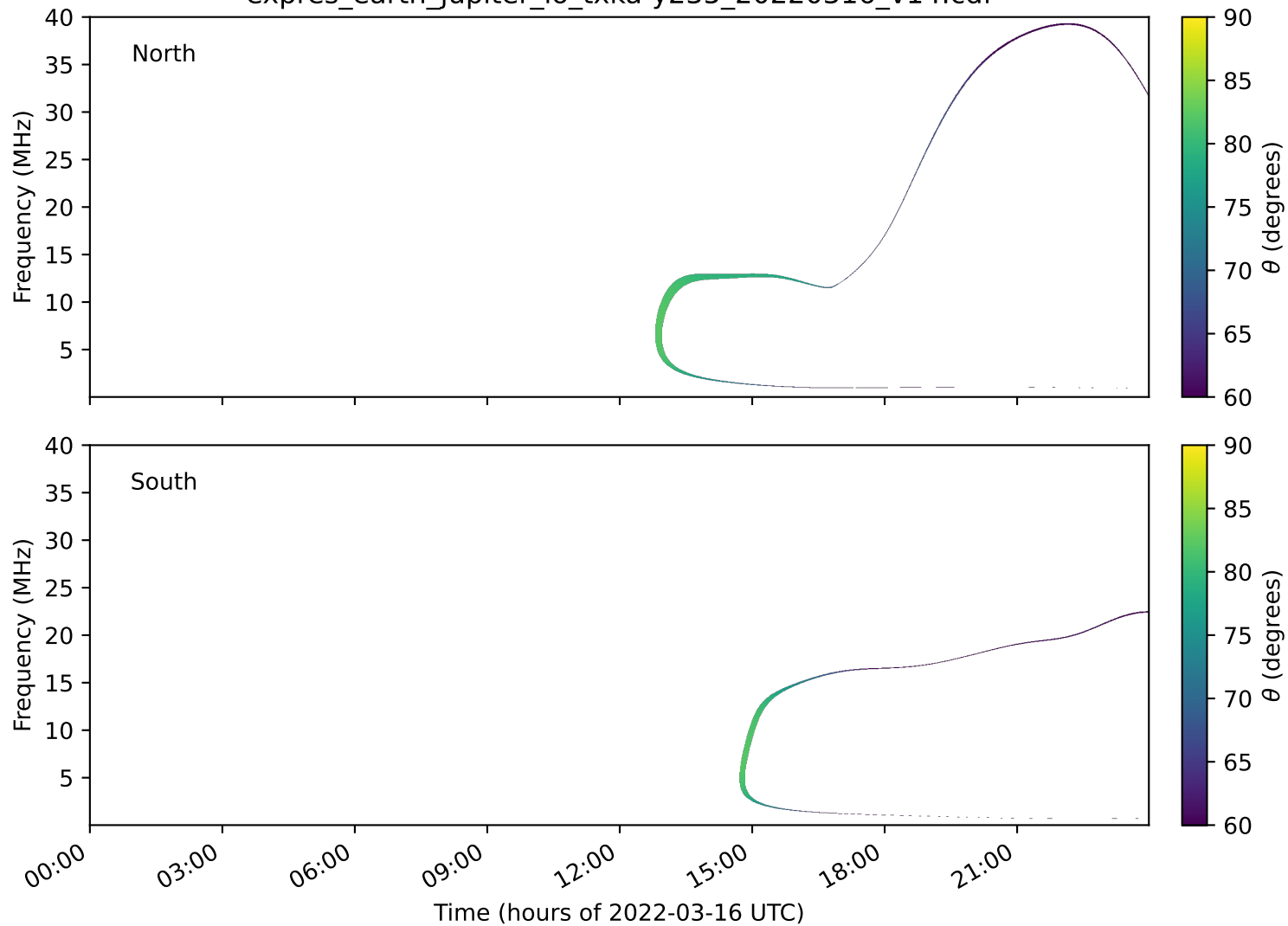
expres_earth_jupiter_io_txka-y235_20220316_v14.cdf
