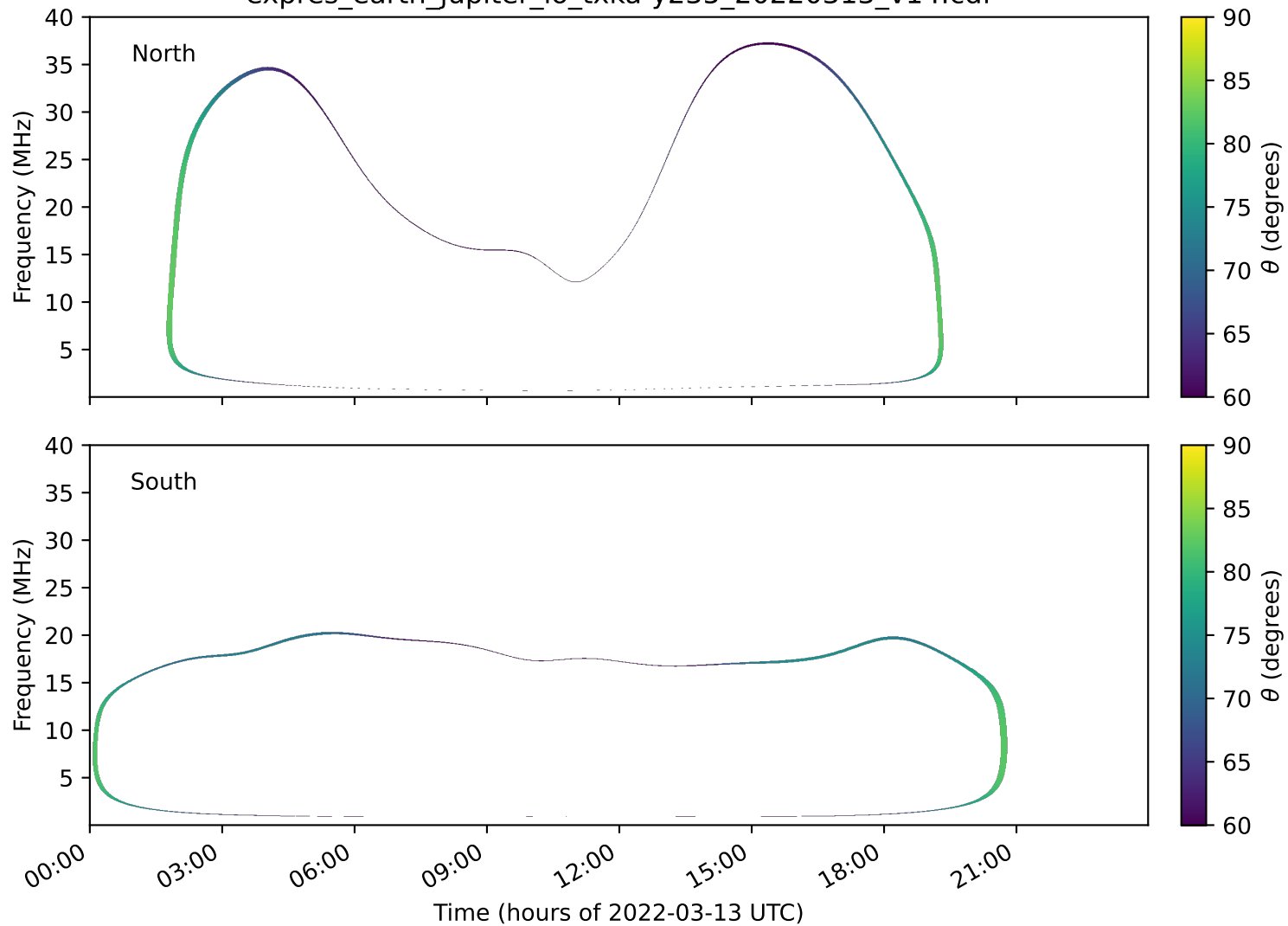
expres_earth_jupiter_io_txka-y235_20220313_v14.cdf
