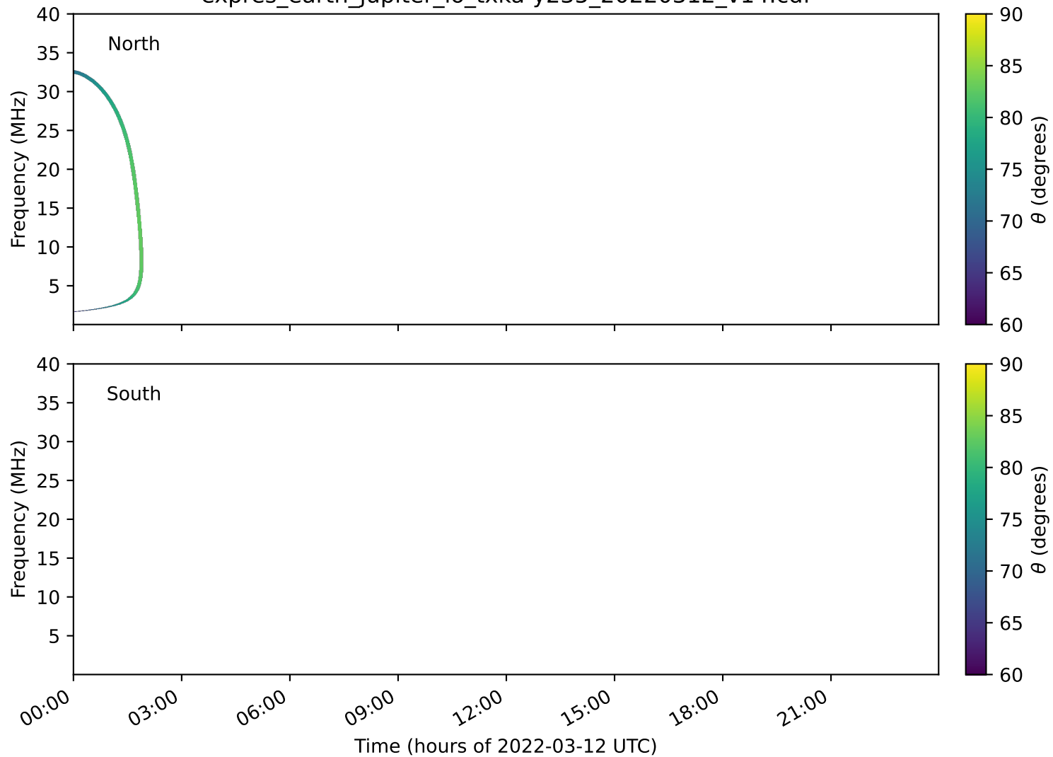
expres_earth_jupiter_io_txka-y235_20220312_v14.cdf
