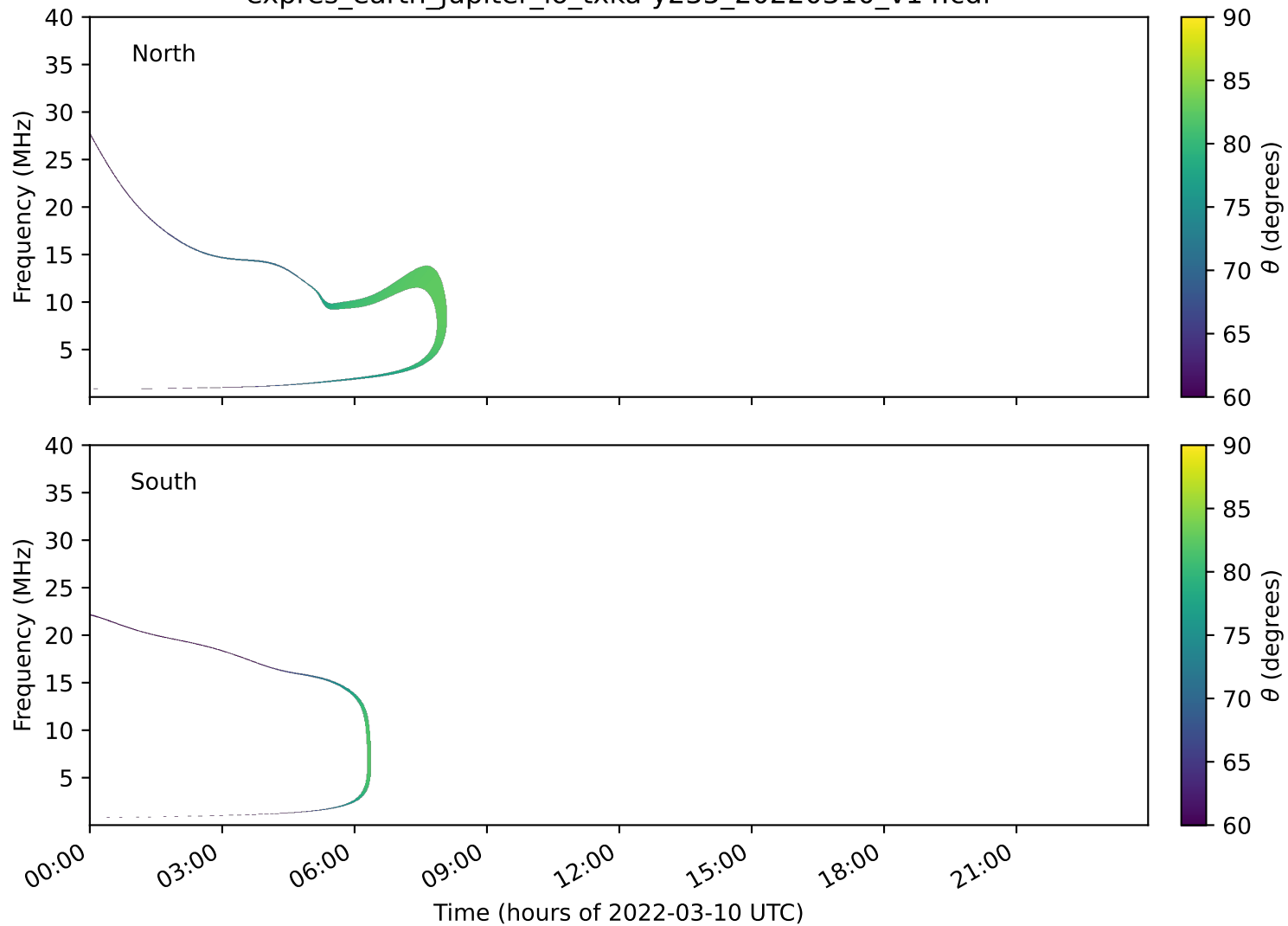
expres_earth_jupiter_io_txka-y235_20220310_v14.cdf
