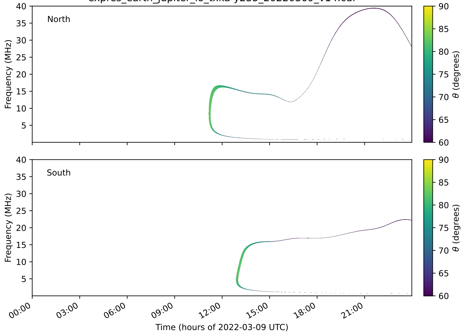
expres_earth_jupiter_io_txka-y235_20220309_v14.cdf
