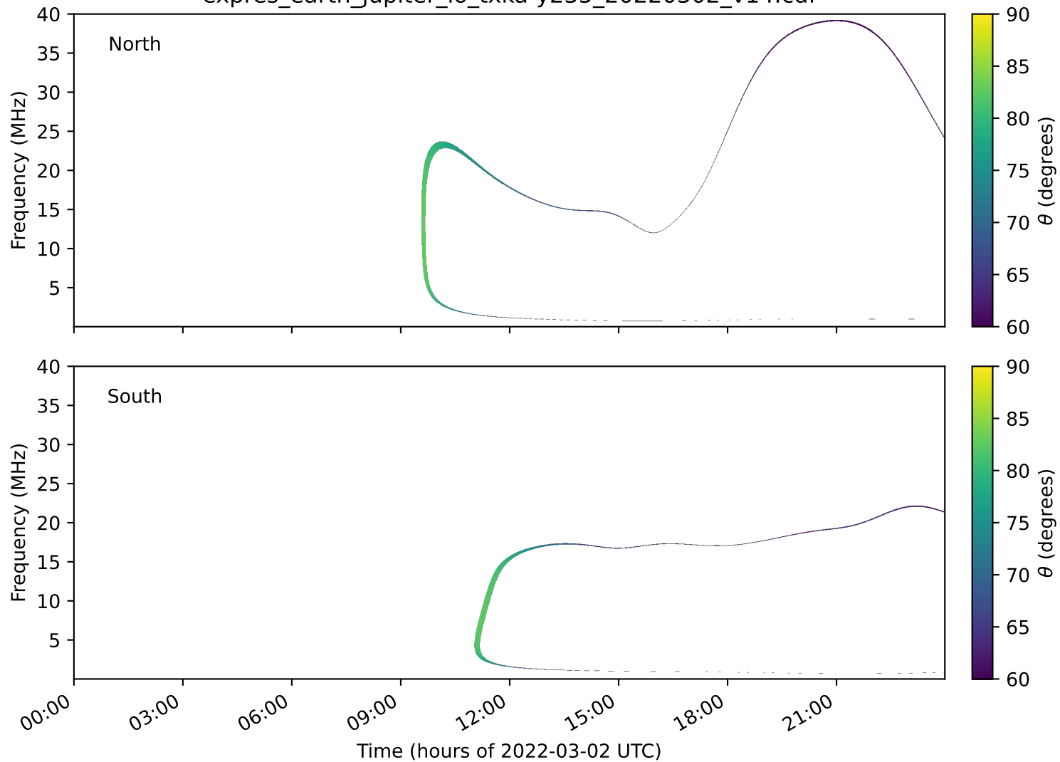
expres_earth_jupiter_io_txka-y235_20220302_v14.cdf
