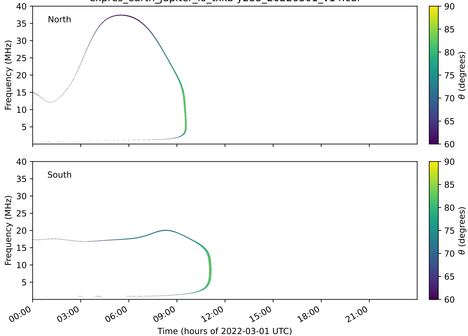
expres_earth_jupiter_io_txka-y235_20220301_v14.cdf
