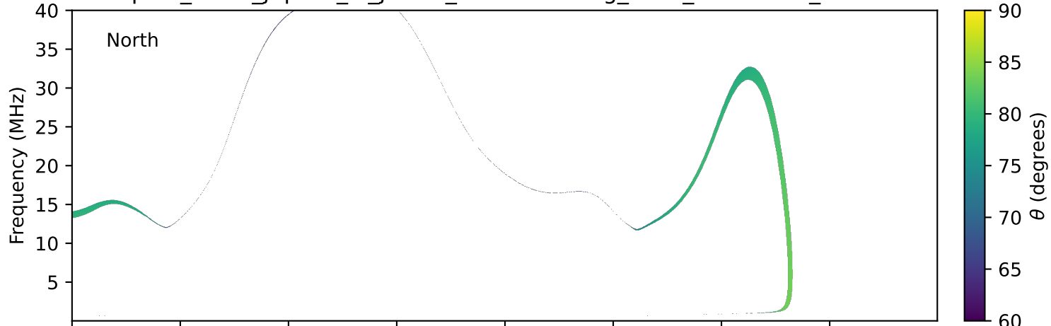
expres_earth_jupiter_io_jrm33_lossc-wid1deg_3kev_20220329_v11.cdf
