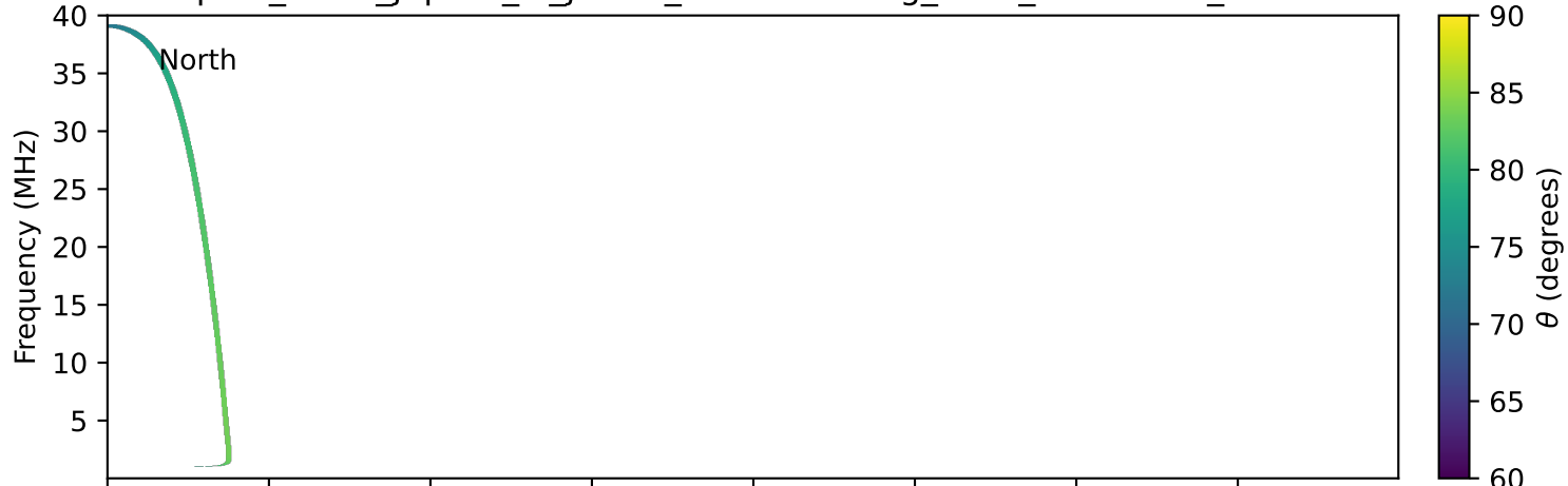
expres_earth_jupiter_io_jrm33_lossc-wid1deg_3kev_20220312_v11.cdf
