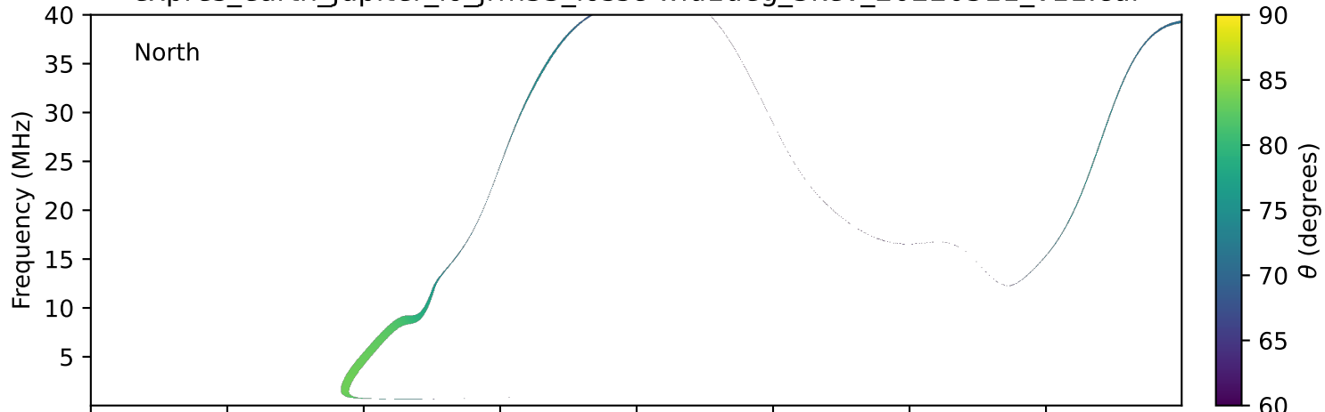
expres_earth_jupiter_io_jrm33_lossc-wid1deg_3kev_20220311_v11.cdf
