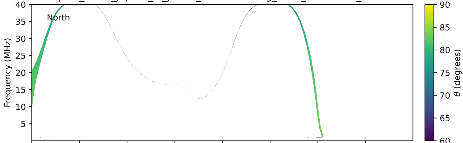
expres_earth_jupiter_io_jrm33_lossc-wid1deg_3kev_20220306_v11.cdf
