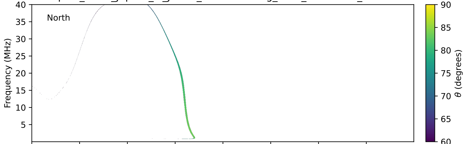
expres_earth_jupiter_io_jrm33_lossc-wid1deg_3kev_20220301_v11.cdf
