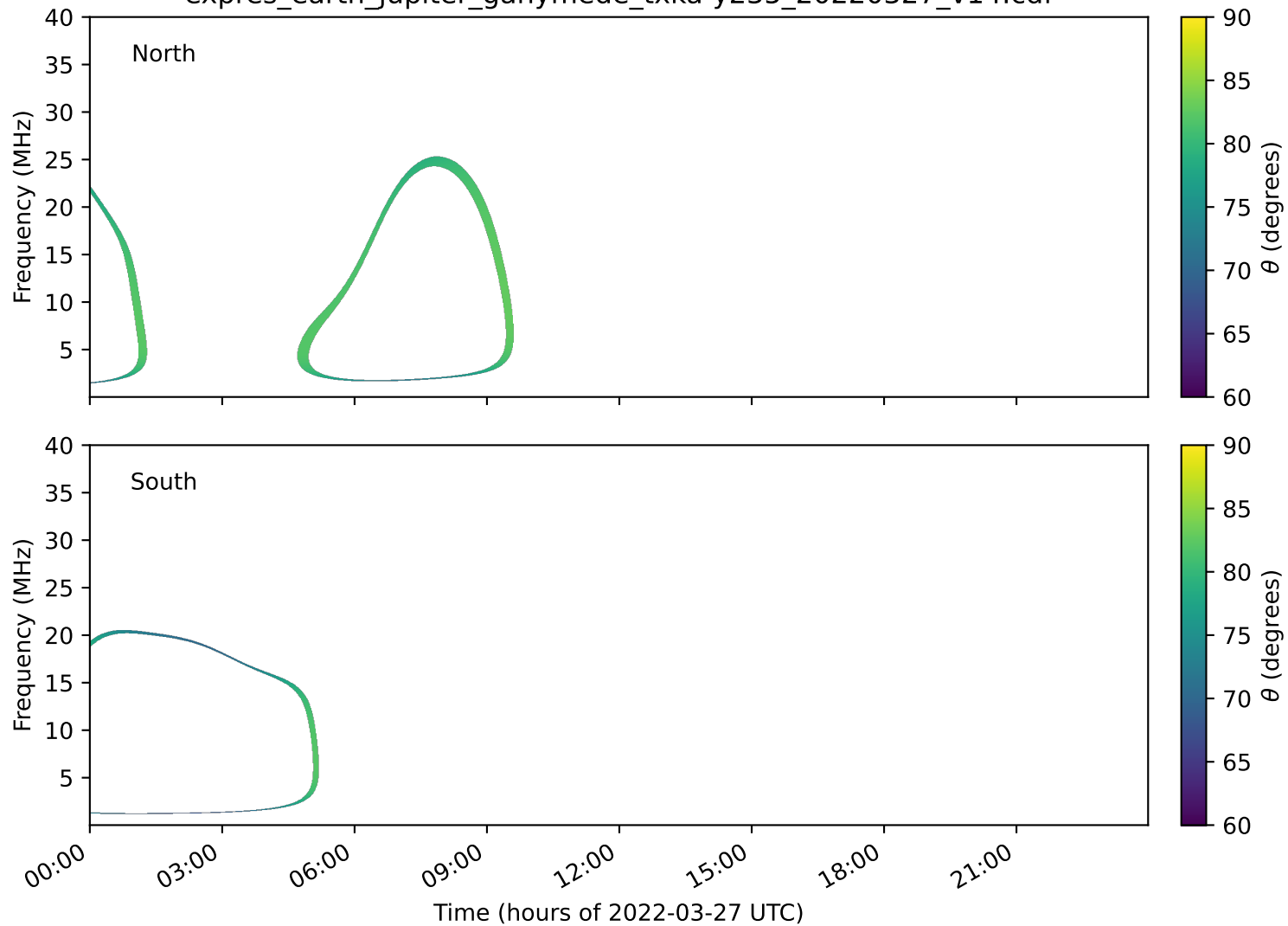
expres_earth_jupiter_ganymede_txka-y235_20220327_v14.cdf
