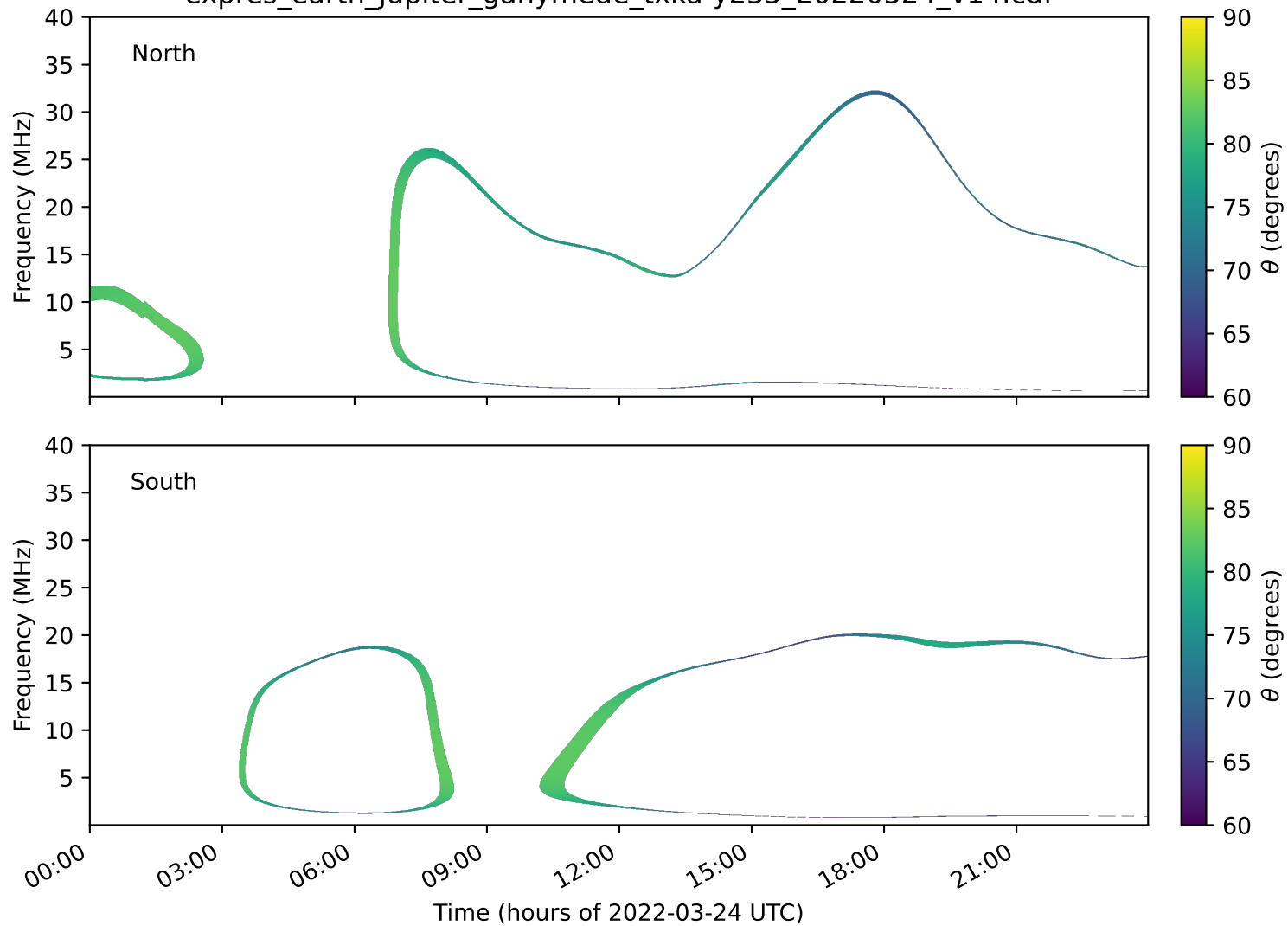
expres_earth_jupiter_ganymede_txka-y235_20220324_v14.cdf
