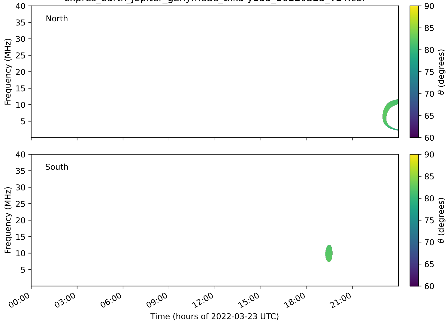
expres_earth_jupiter_ganymede_txka-y235_20220323_v14.cdf
