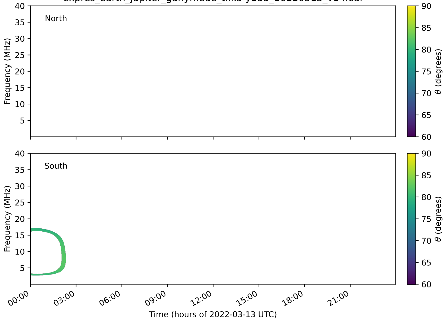
expres_earth_jupiter_ganymede_txka-y235_20220313_v14.cdf
