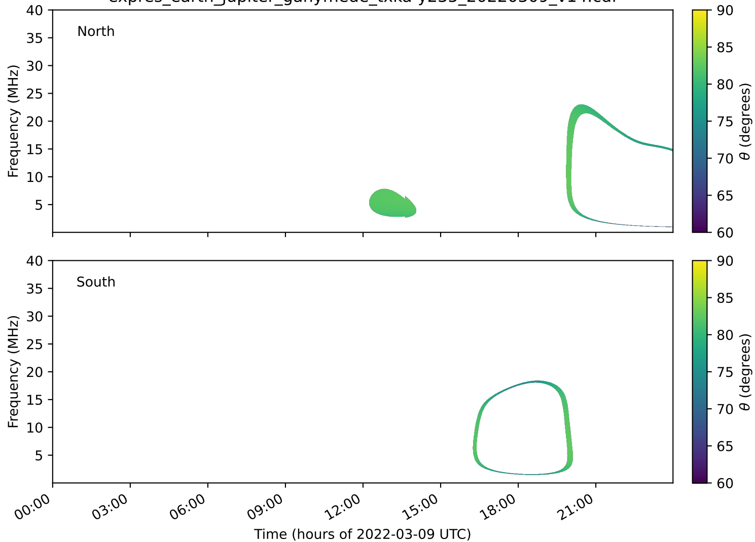
expres_earth_jupiter_ganymede_txka-y235_20220309_v14.cdf
